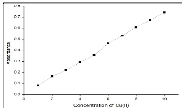
Figure 1. Calibration plot of Cu (II) with BIZPINPH
