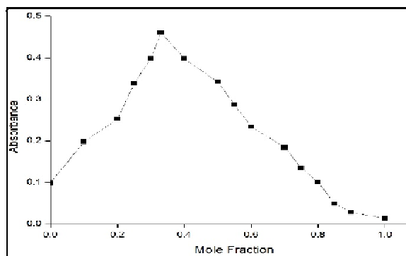
Figure 2. Job's continuous variation method
